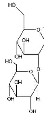
IV ( \beta -D-glucopyranosyl- \beta -D-glucopyranosyl)
